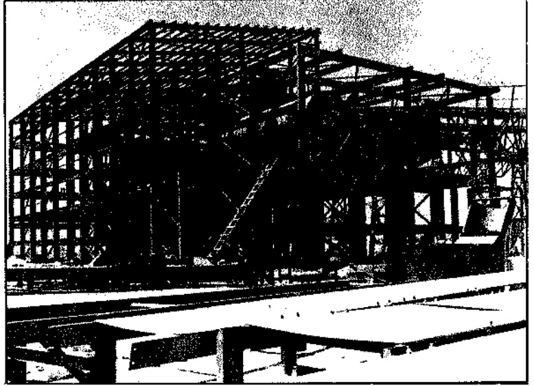
ETİBANK-MAZIDAĞI PHOSPHATE PLANT/MARDİN
